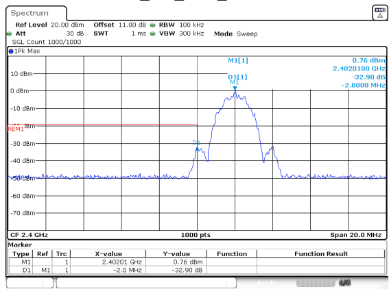
BLE_2M_Low_Channel
