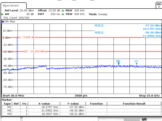
BLE_2M_Low_Channel
