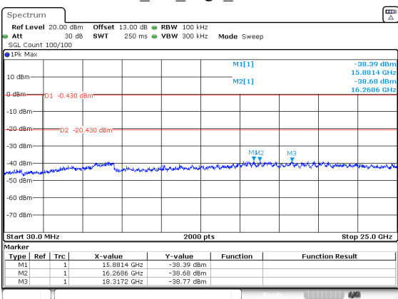
BLE_2M_High_Channel
