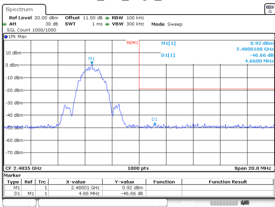
BLE_2M_High_Channel
