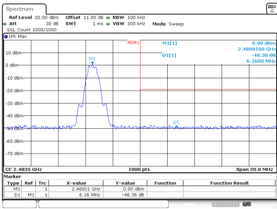
BLE_1M_High_Channel
