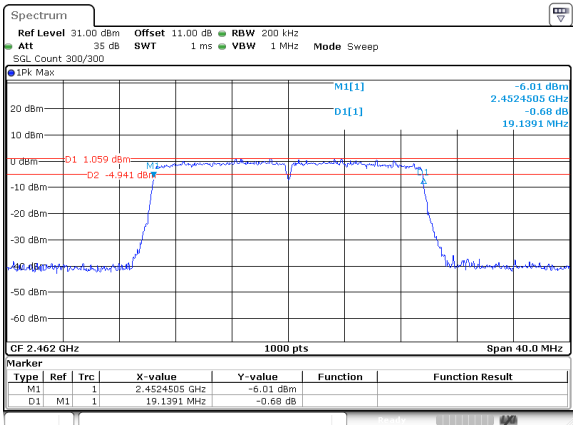
802.11ax20_2462MHz_RU_FULL_Chain 1
