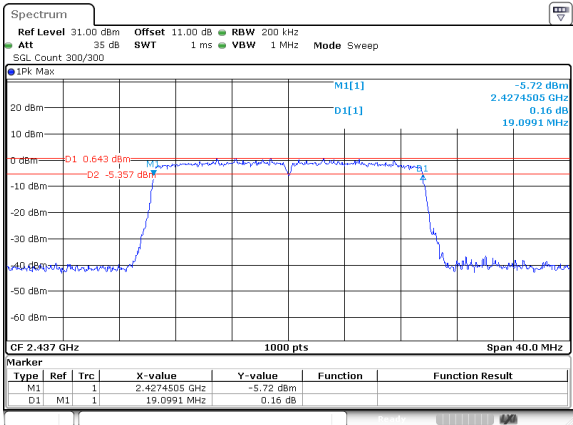
802.11ax20_2437MHz_RU_FULL_Chain 0
