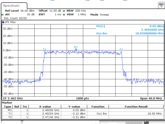
802.11ax20_2462MHz_RU_FULL_Chain 1
