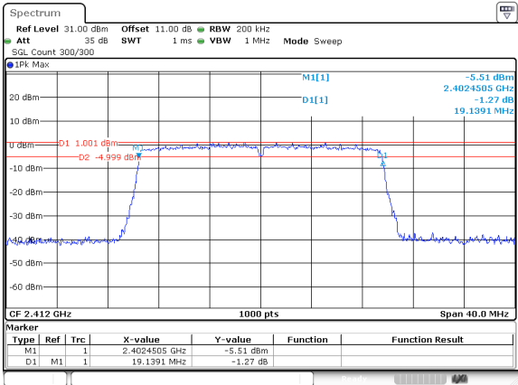
802.11ax20_2412MHz_RU_FULL_Chain 1
