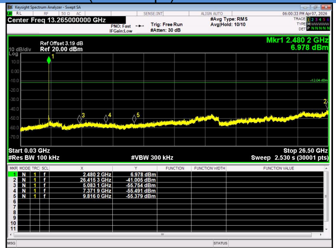
GFSK(BLE 1Mbps) HIGH CHANNEL
