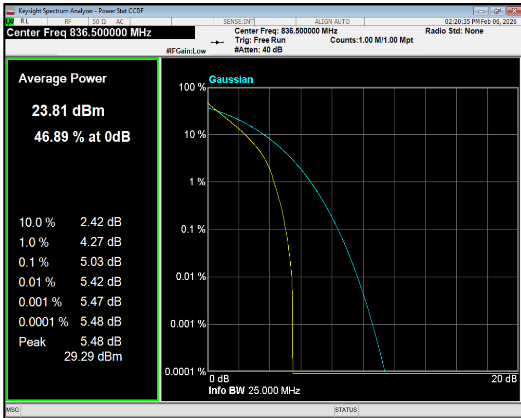
Band5 QPSK BW=1.4MHz Channel=20525 RB Size=3 Position=#Max
