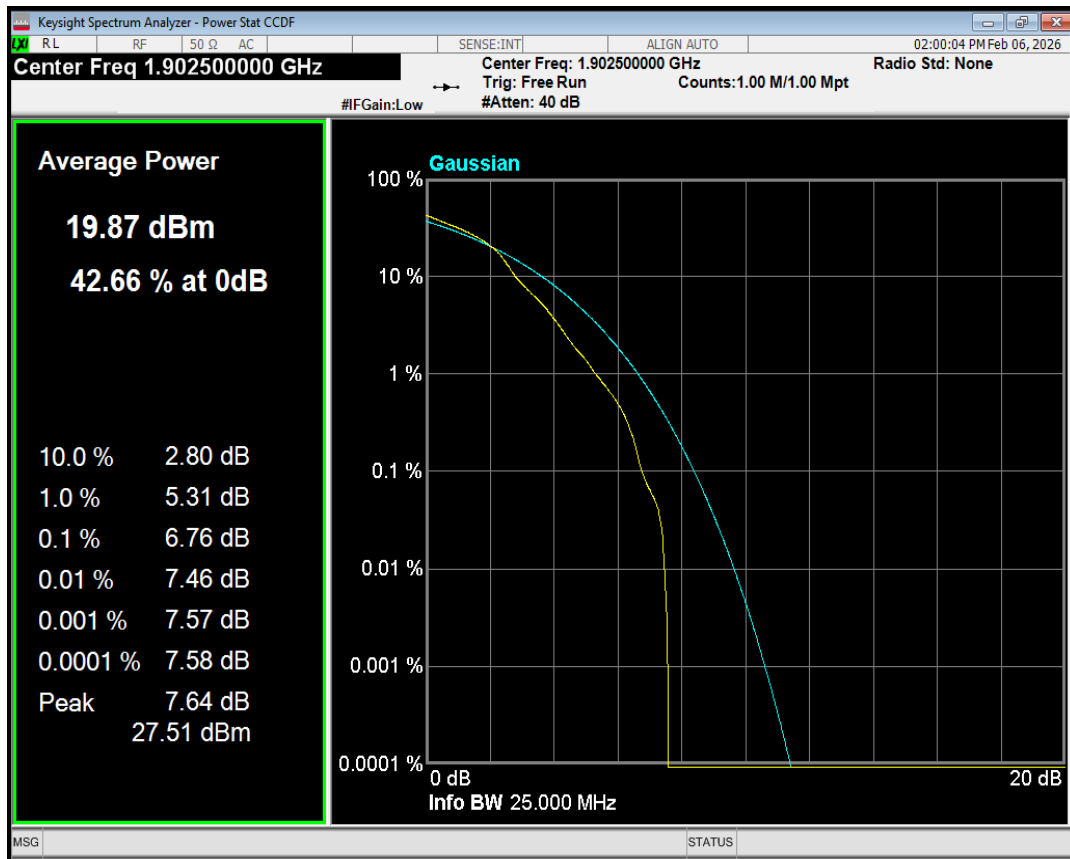
Band2 QAM16 BW=15MHz Channel=19125 RB Size=1 Position=#Mid
