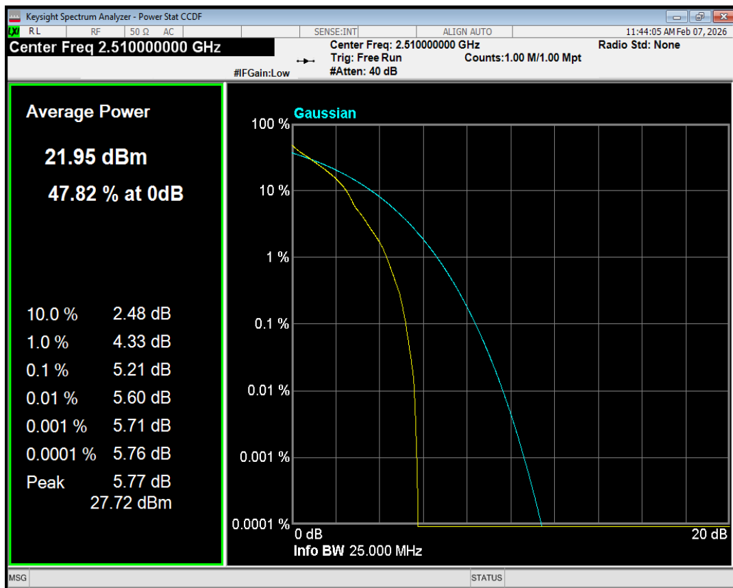
Band7 QPSK BW=20MHz Channel=20850 RB Size=50 Position=#0
