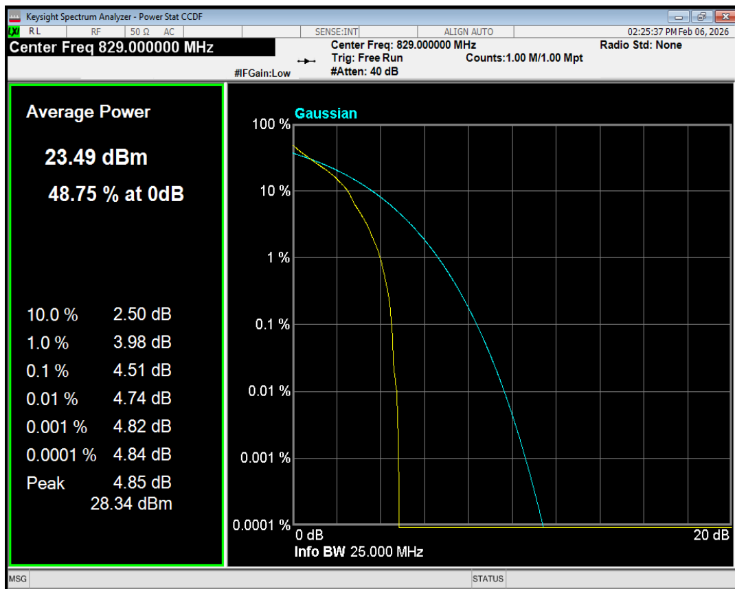
Band5 QPSK BW=10MHz Channel=20450 RB Size=25 Position=#0
