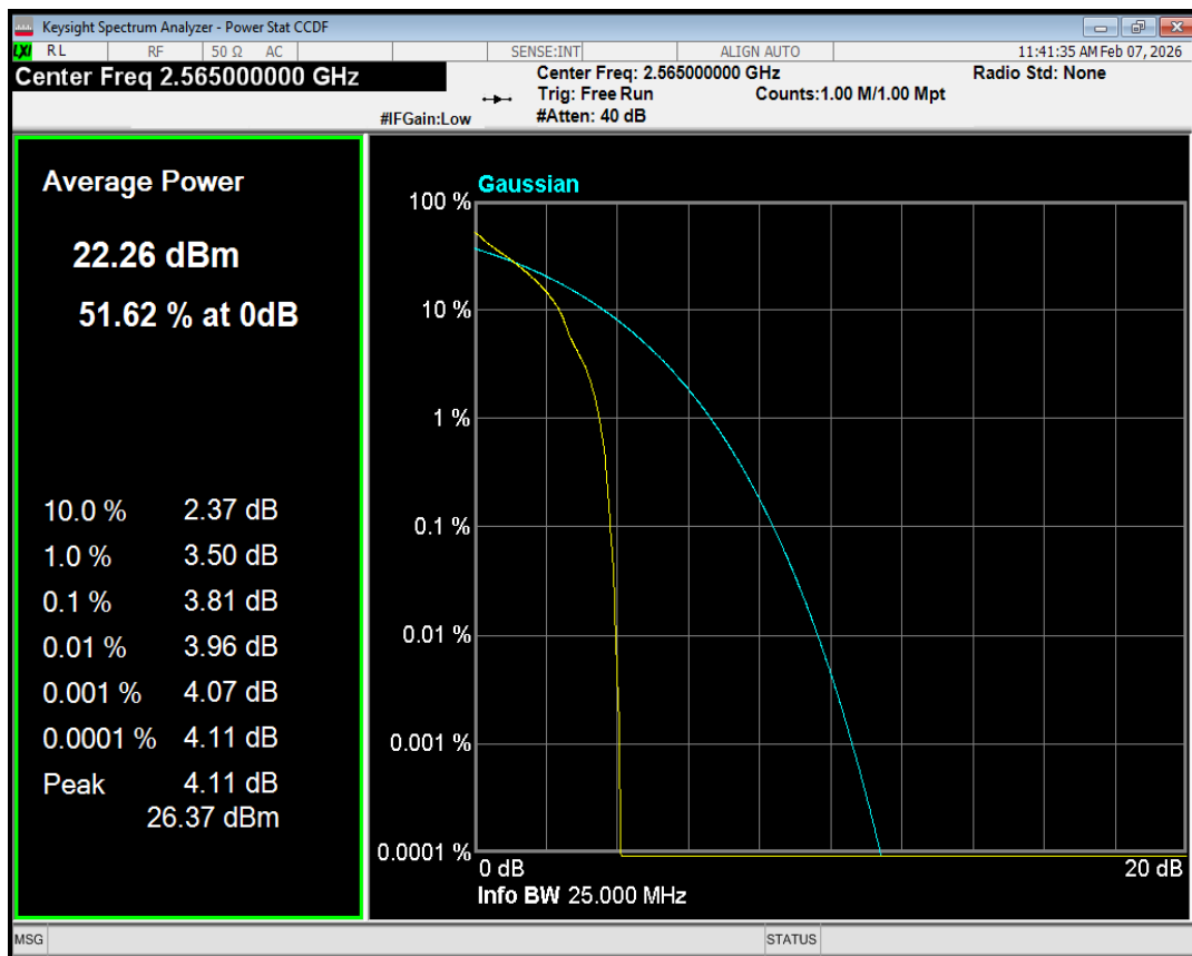
Band7 QPSK BW=10MHz Channel=21400 RB Size=25 Position=#0
