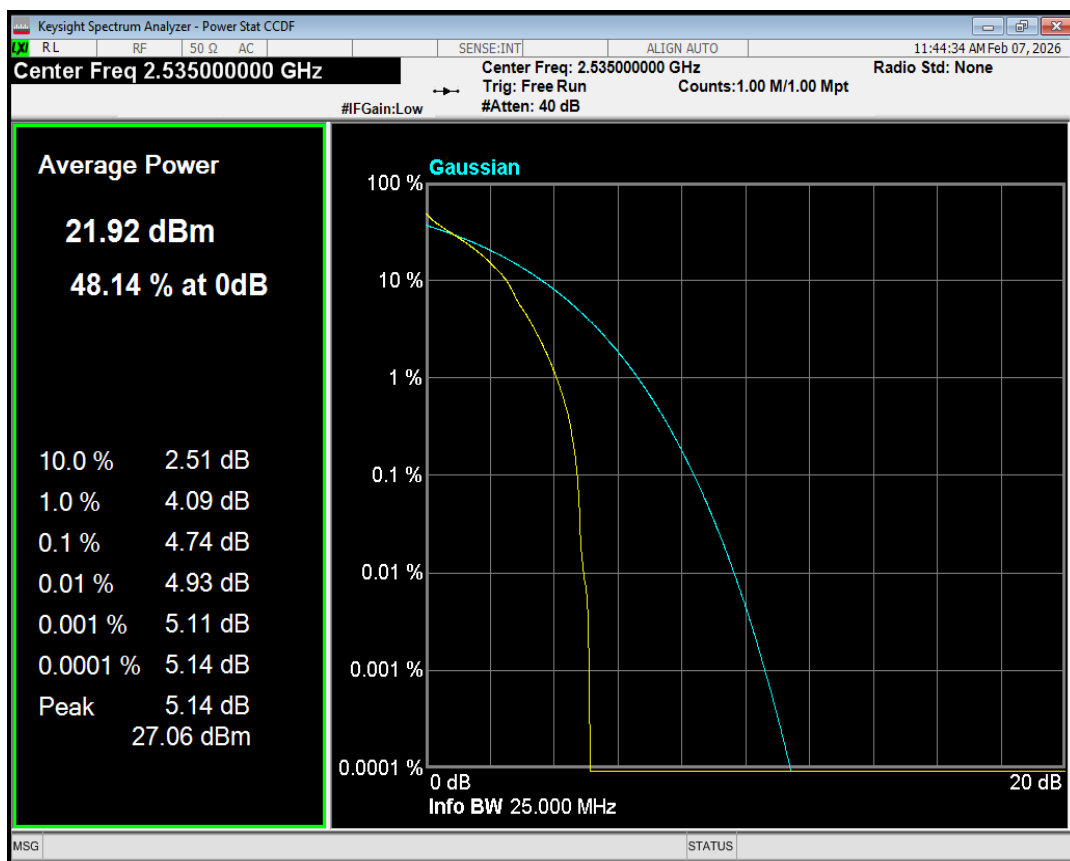
Band7 QPSK BW=20MHz Channel=21100 RB Size=1 Position=#Mid
