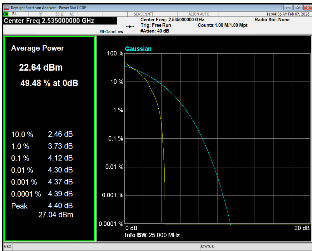
Band7 QPSK BW=20MHz Channel=21100 RB Size=1 Position=#Max
