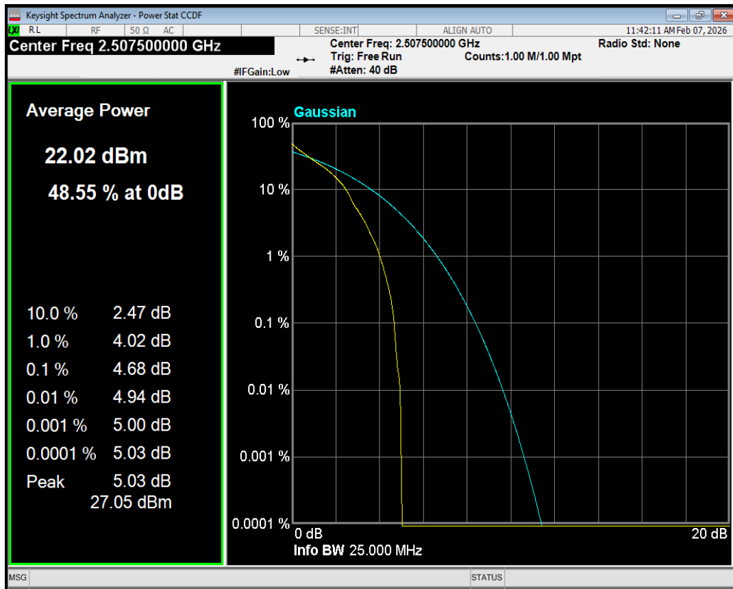
Band7 QPSK BW=15MHz Channel=20825 RB Size=1 Position=#Mid
