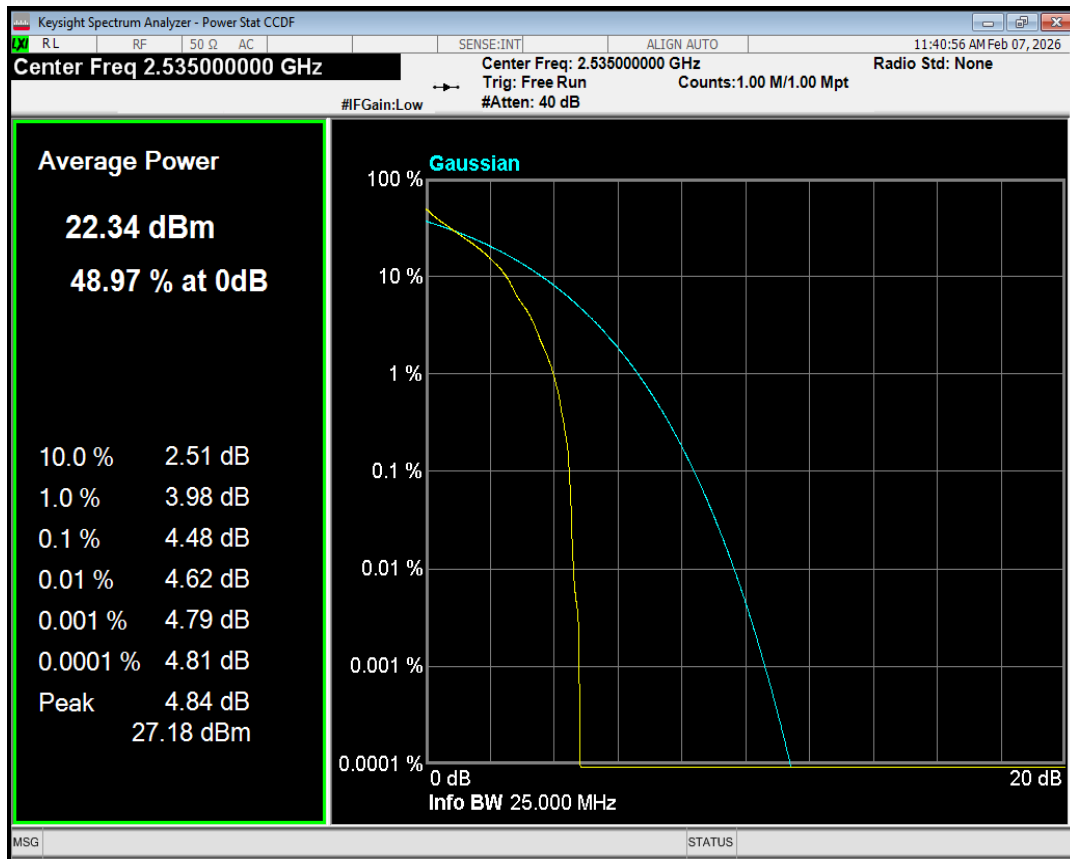
Band7 QPSK BW=10MHz Channel=21100 RB Size=1 Position=#Mid
