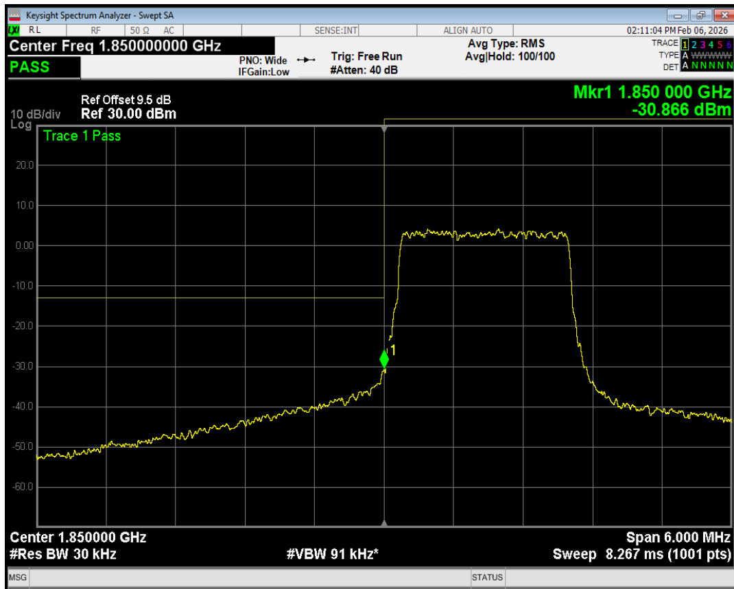
Band2 QAM16 BW=3MHz Channel=18615 RB Size=8 Position=#Max
