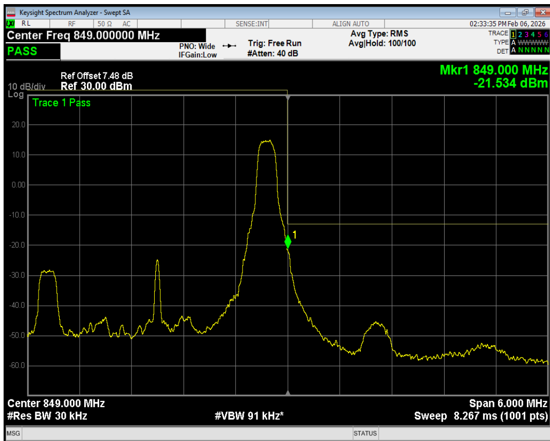
Band5 QAM16 BW=3MHz Channel=20635 RB Size=8 Position=#0
