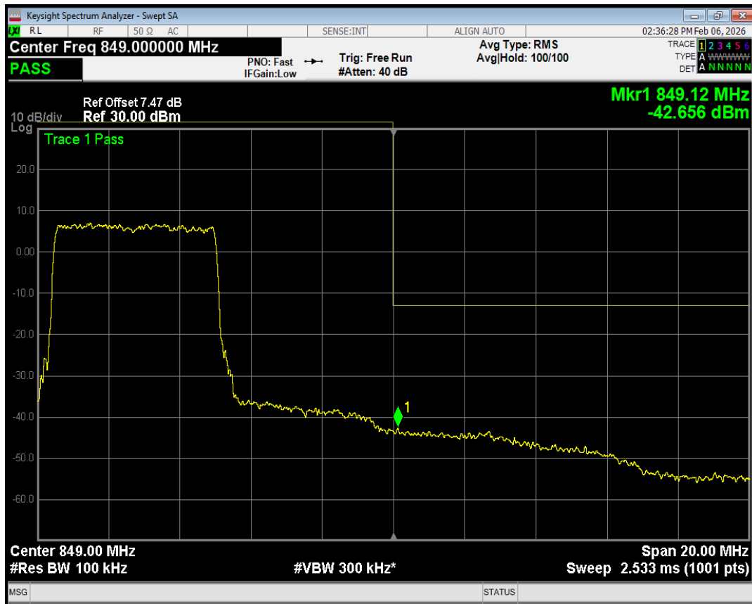
Band5 QPSK BW=10MHz Channel=20600 RB Size=25 Position=#Max
