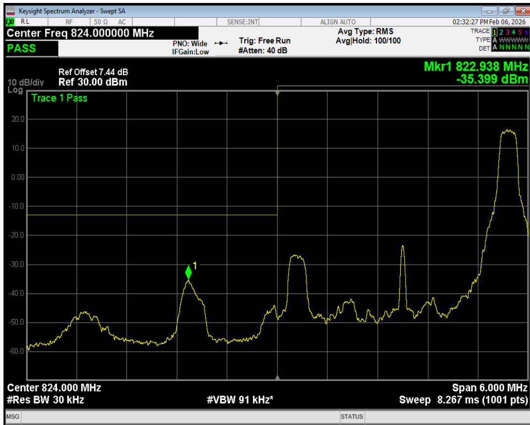
Band5 QPSK BW=3MHz Channel=20415 RB Size=8 Position=#0
