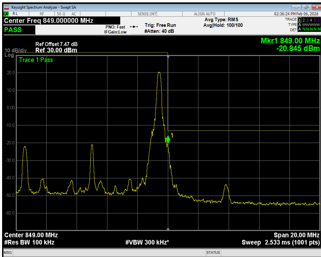
Band5 QPSK BW=10MHz Channel=20600 RB Size=25 Position=#0
