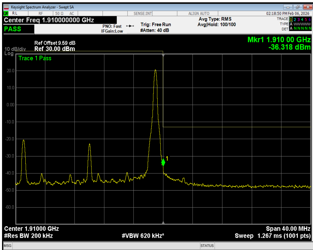
Band2 QPSK BW=20MHz Channel=19100 RB Size=50 Position=#0
