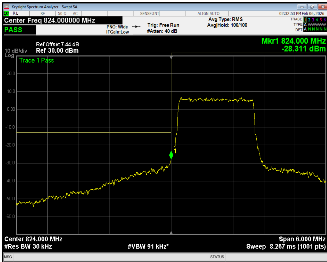
Band5 QAM16 BW=3MHz Channel=20415 RB Size=8 Position=#Max
