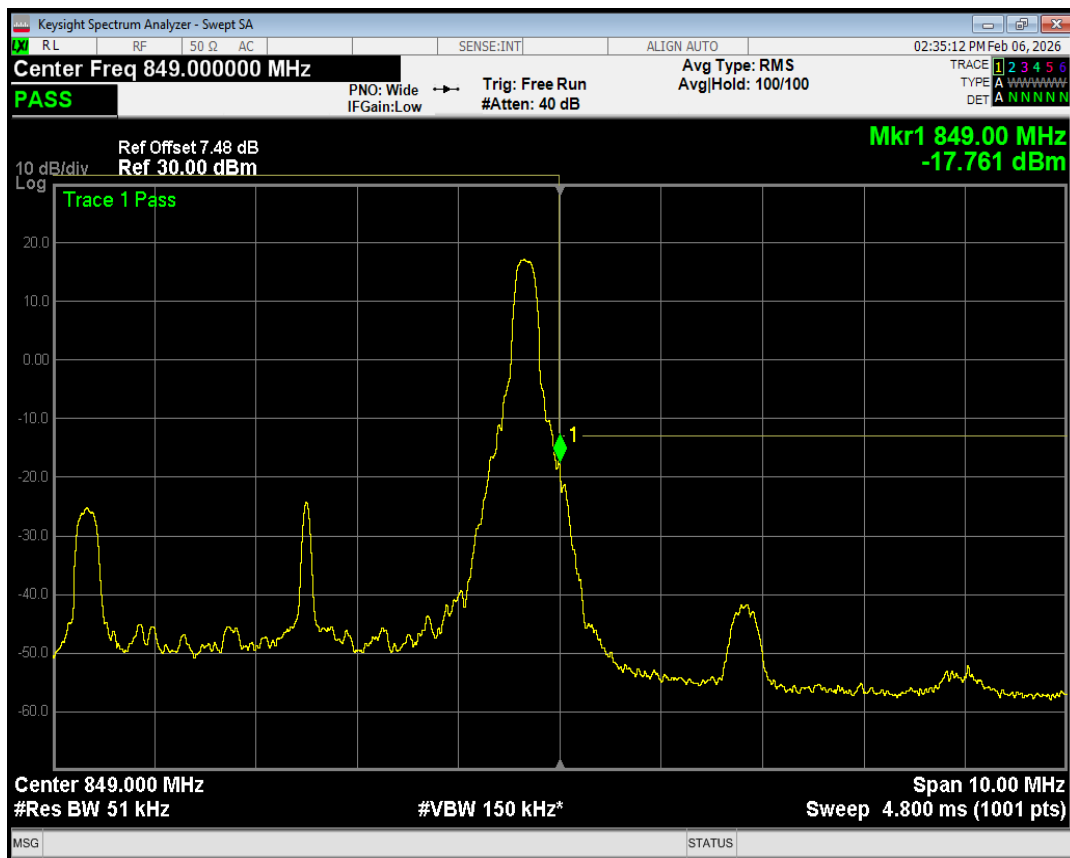
Band5 QAM16 BW=5MHz Channel=20625 RB Size=12 Position=#0
