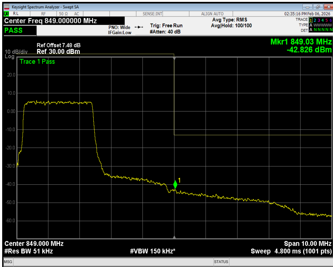
Band5 QAM16 BW=5MHz Channel=20625 RB Size=12 Position=#Max
