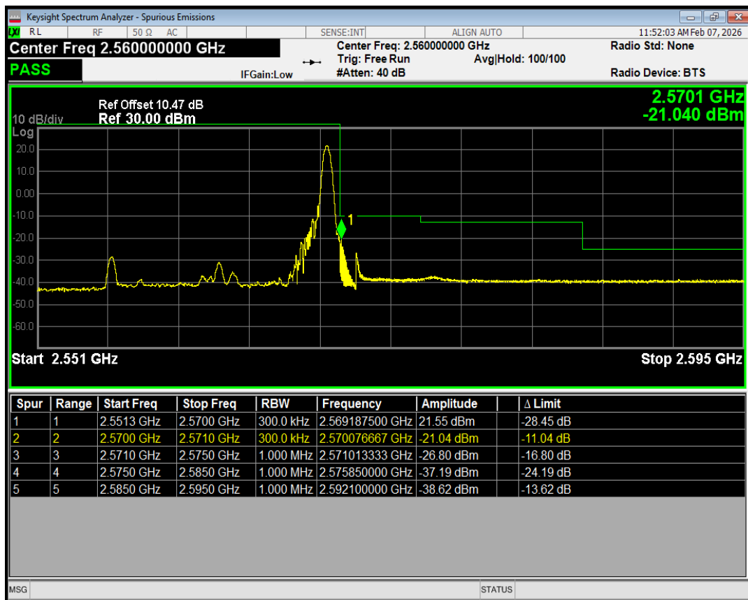
Band7 QPSK BW=15MHz Channel=21375 RB Size=36 Position=#0
