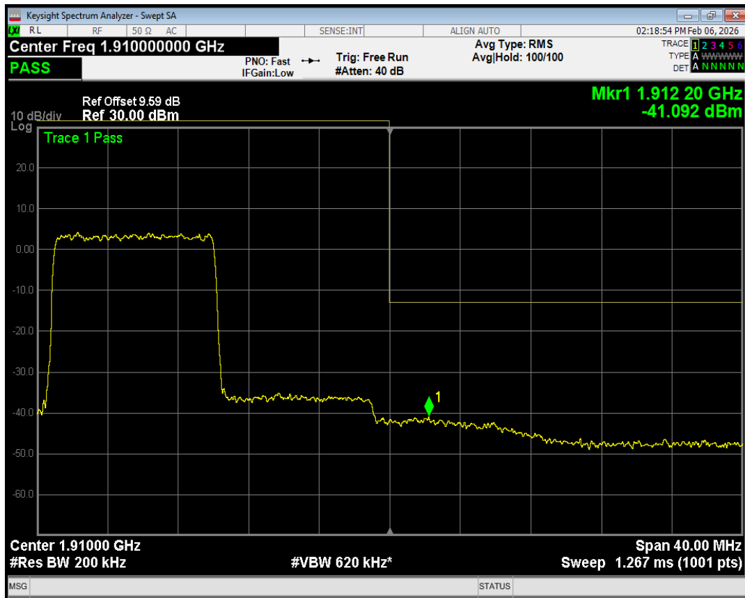
Band2 QPSK BW=20MHz Channel=19100 RB Size=50 Position=#Max
