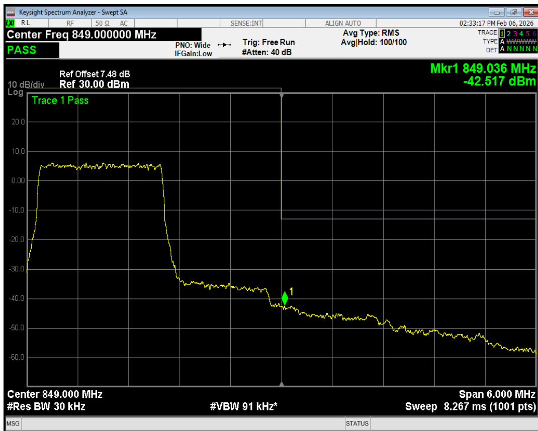
Band5 QPSK BW=3MHz Channel=20635 RB Size=8 Position=#Max
