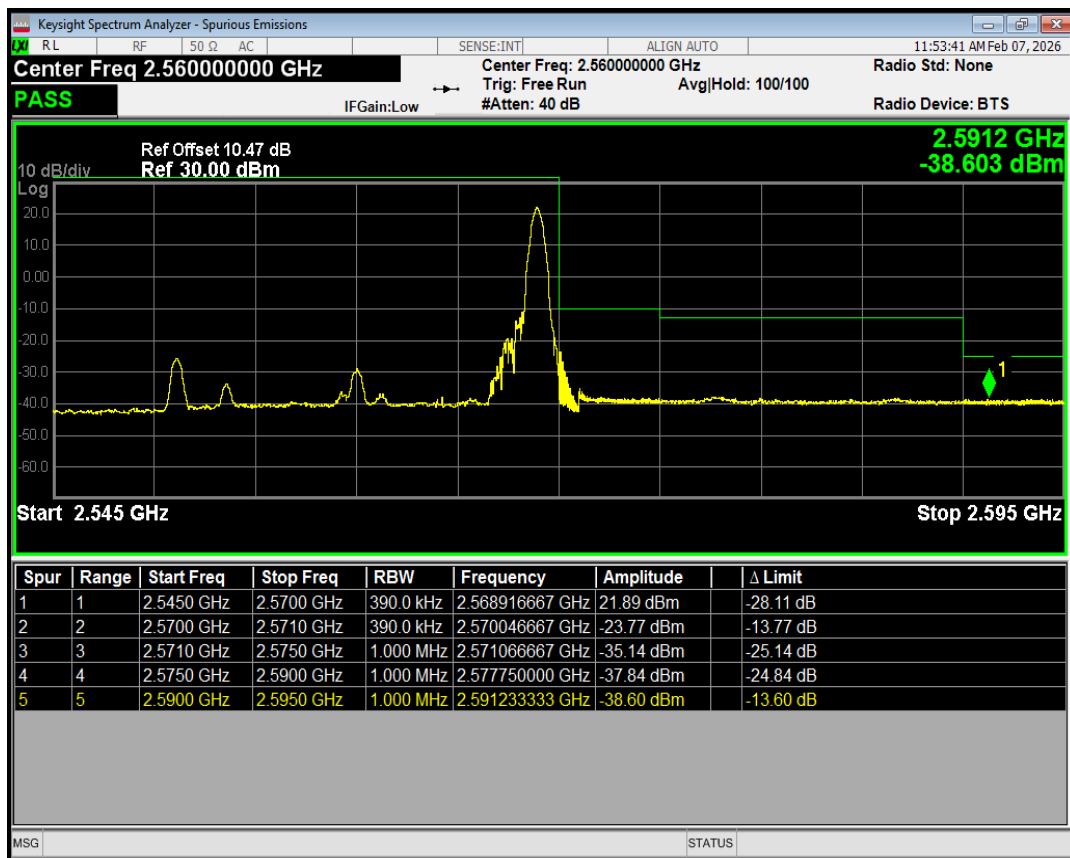
Band7 QPSK BW=20MHz Channel=21350 RB Size=50 Position=#0
