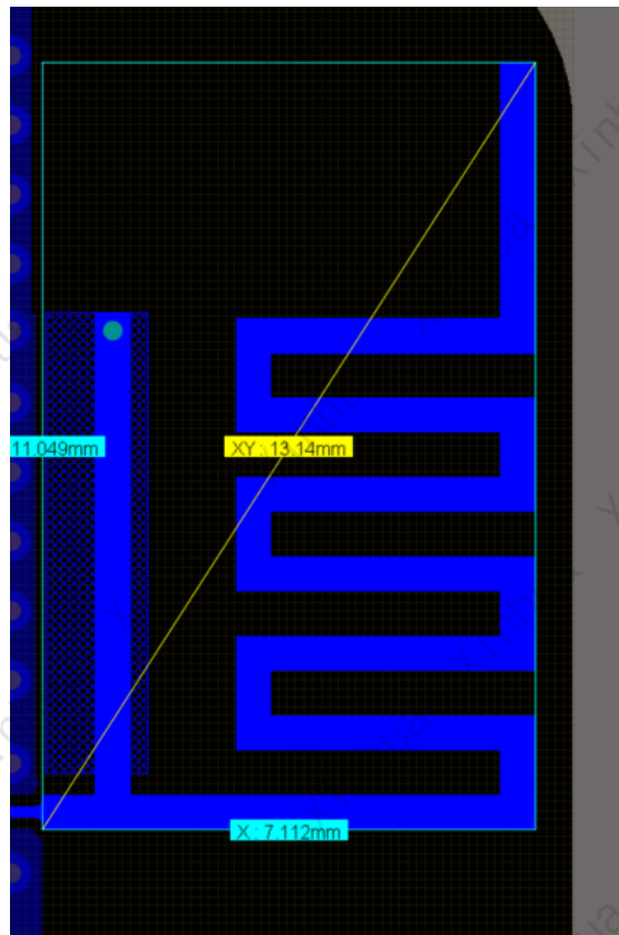
Antenna Dimensions
