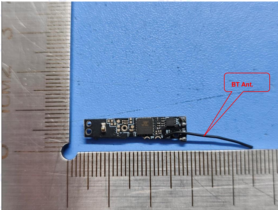
Photo 10 Appearance of PCB (Left)
