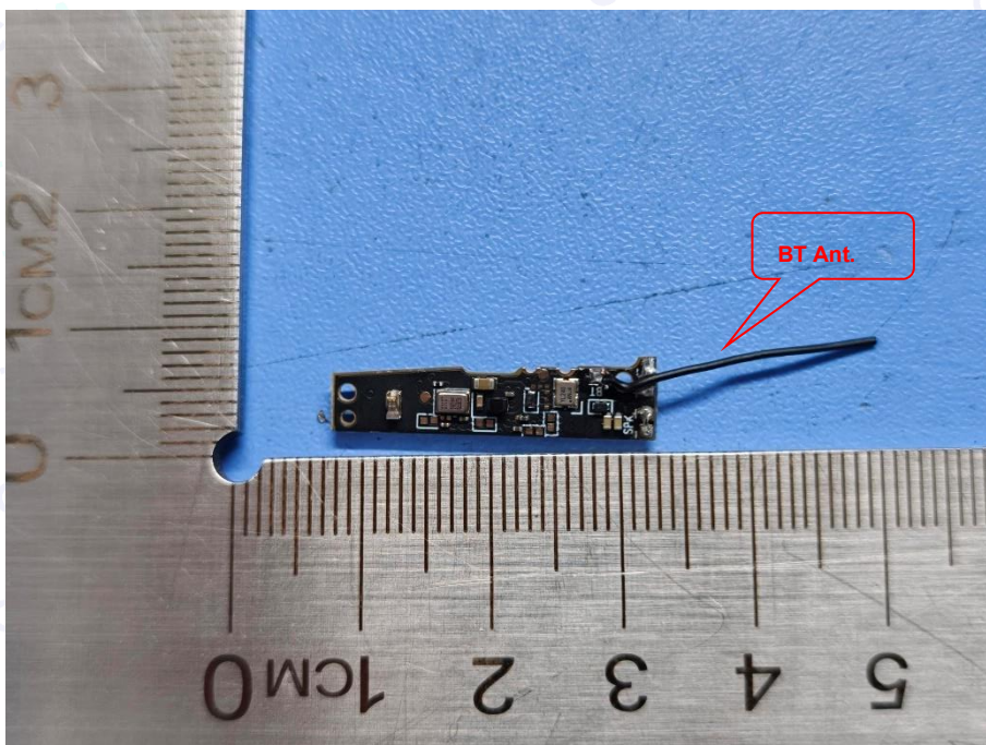
Photo 8 Appearance of PCB (Right)
