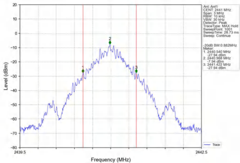
GFSK_DH5_MCH_2441MHz_Ant1_NTNV
