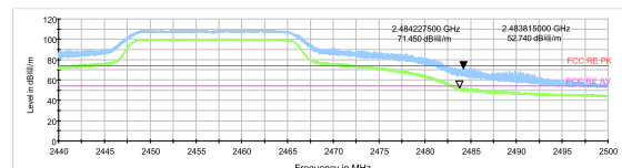
802.11n HT20 -Channel 10 Peak+ Average
