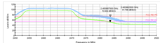
802.11g-Channel 11 Peak+ Average
