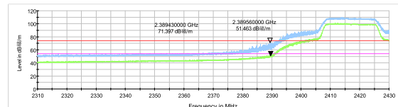
802.11n HT20 -Channel 2 Peak+ Average
