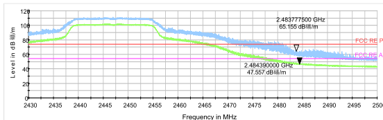
802.11g-Channel 8 Peak+ Average
