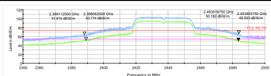
802.11n HT40 -Channel 6 Peak+ Average
