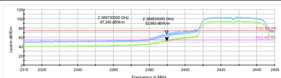
802.11n HT40 -Channel 4 Peak+ Average
