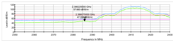
802.11b-Channel 1 Peak+ Average
