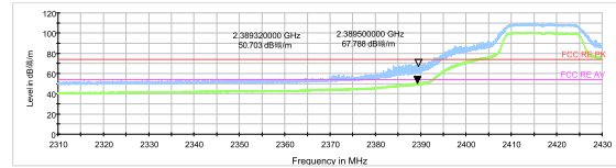
802.11g-Channel 2 Peak+ Average
