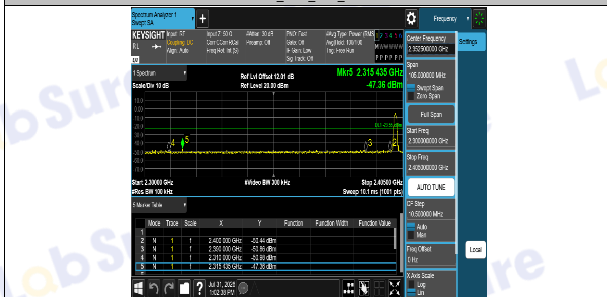
2DH5_Ant1_Low_2402
