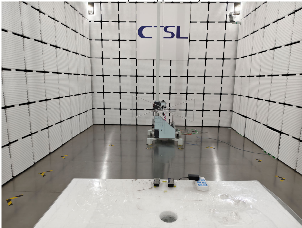
Photo 1 Test Setup Photos of Radiated Emission Test (30-1000MHz) Switch Power Adapter supported by the Test lab.
