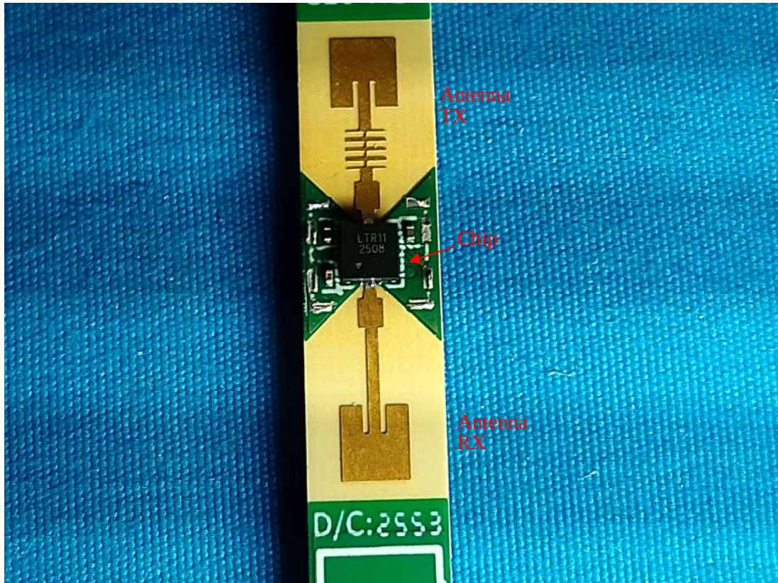
Radar Antenna+Chip
