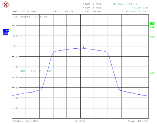
802.11a_5300MHz
