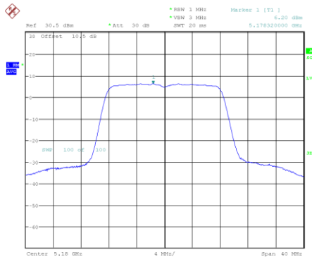
802.11a_5180MHz
