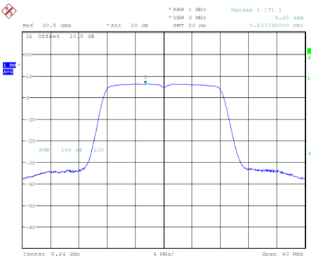
802.11a_5240MHz
