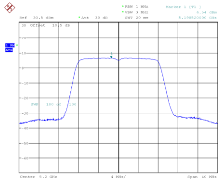
802.11a_5200MHz
