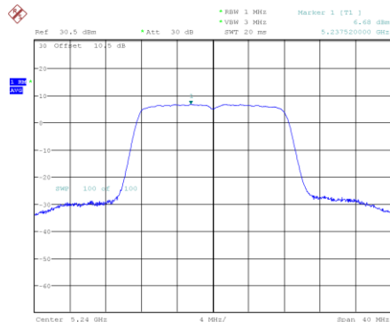
802.11a_5240MHz
