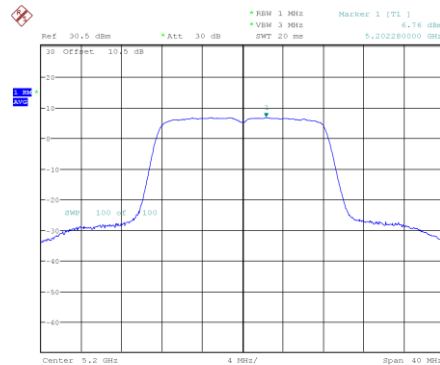
802.11a_5200MHz
