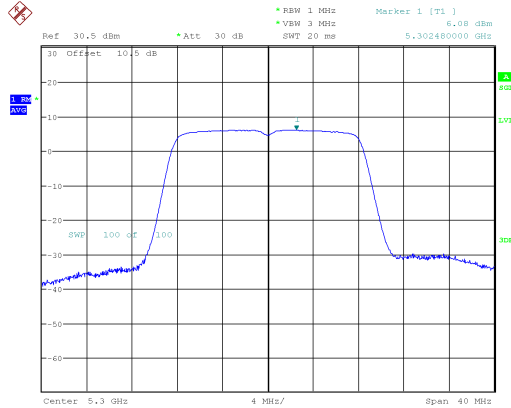
802.11a_5300MHz
