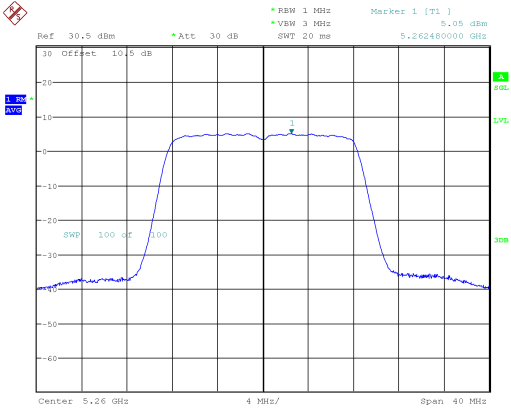
802.11a_5260MHz
