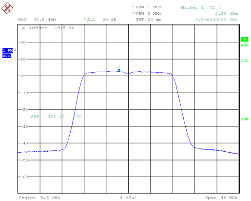
802.11a_5600MHz
