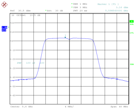
802.11a_5600MHz
