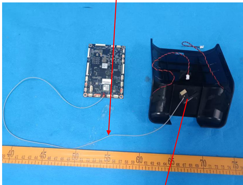
View of RF antenna
