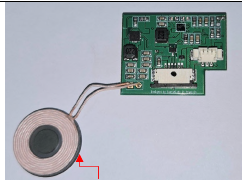
Coil Antenna
