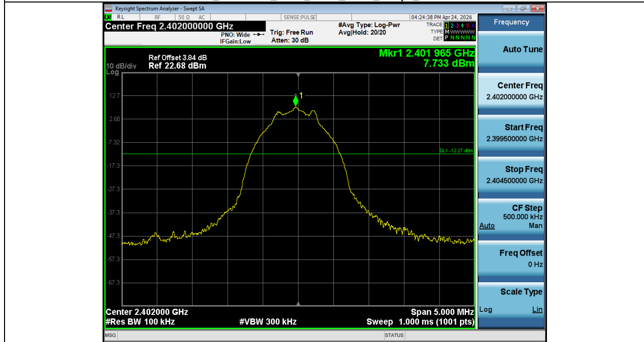
2 Bandedge_NVNT_ANT1_1Mbps_2402
