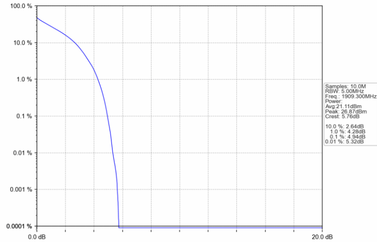
Band2_1.4MHz_QPSK_HCH_1909.3MHz_RB_6_0_NTNV
