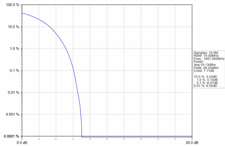
Band2_15MHz_16QAM_LCH_1857.5MHz_RB_27_0_NTNV
