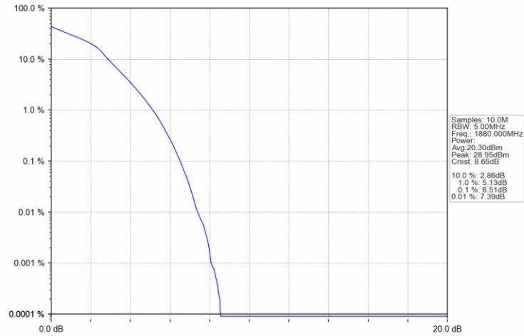
Band2_5MHz_16QAM_MCH_1880MHz_RB_25_0_NTNV
