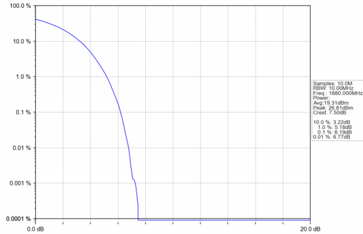
Band2_15MHz_16QAM_MCH_1880MHz_RB_27_0_NTNV
