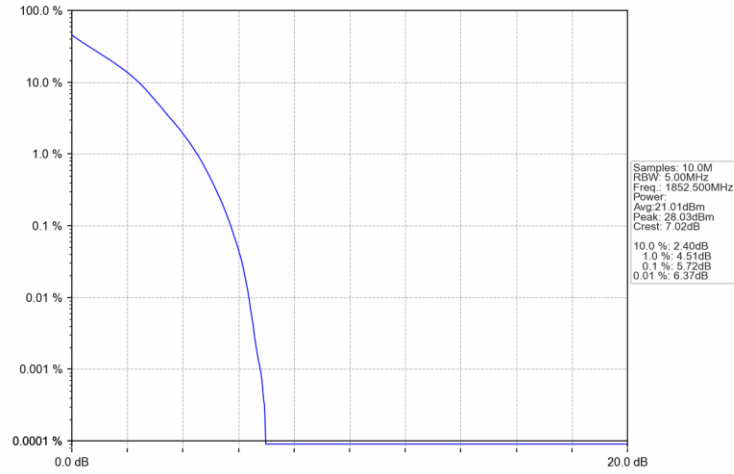
Band2_5MHz_QPSK_LCH_1852.5MHz_RB_25_0_NTNV
