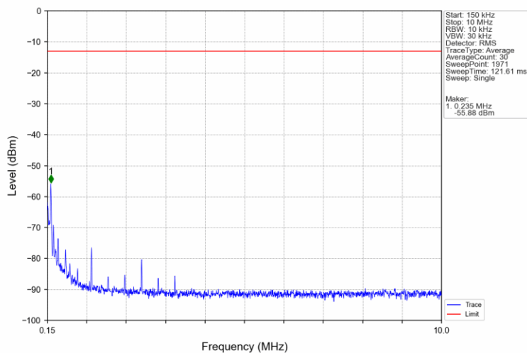
Band2_5MHz_16QAM_MCH_1880MHz_RB_1_0_NTNV
