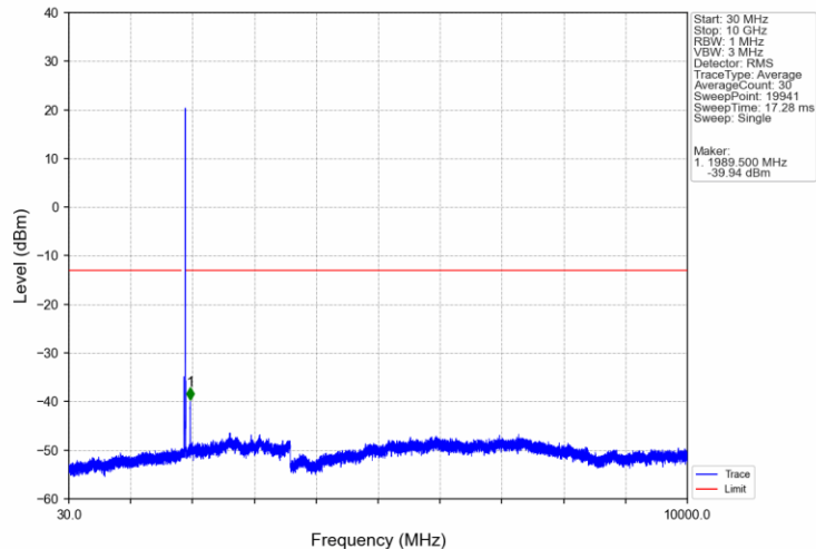
Band2_5MHz_16QAM_HCH_1907.5MHz_RB_1_0_NTNV
