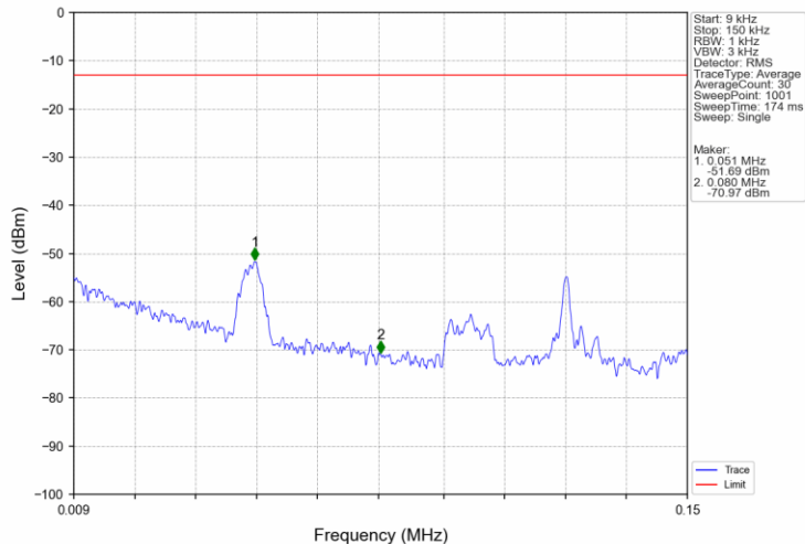
Band2_5MHz_16QAM_MCH_1880MHz_RB_1_0_NTNV
