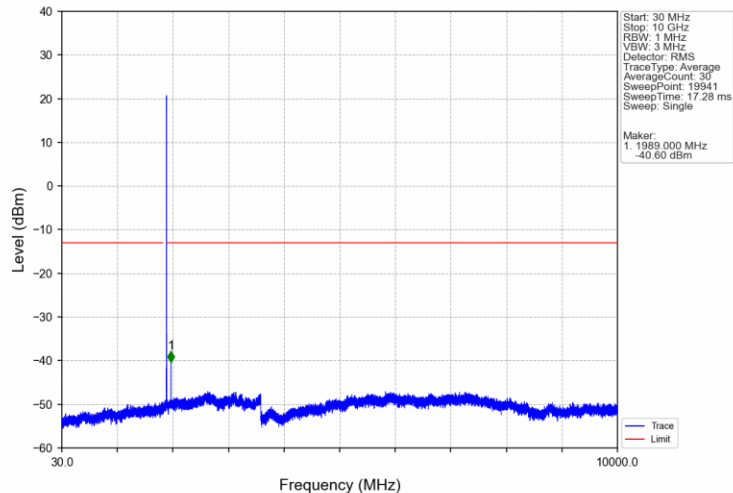
Band2_3MHz_16QAM_HCH_1908.5MHz_RB_1_0_NTNV
