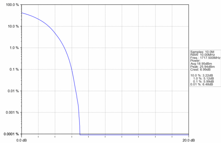
Band4_15MHz_16QAM_LCH_1717.5MHz_RB_27_0_NTNV
