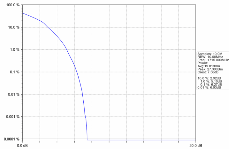
Band4_10MHz_16QAM_LCH_1715MHz_RB_27_0_NTNV
