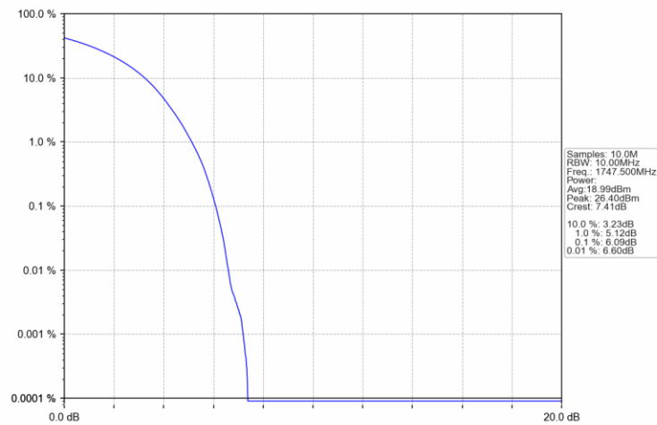
Band4_15MHz_16QAM_HCH_1747.5MHz_RB_27_48_NTNV
