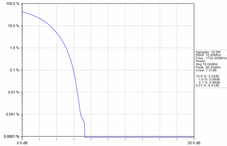
Band4_15MHz_16QAM_MCH_1732.5MHz_RB_27_0_NTNV
