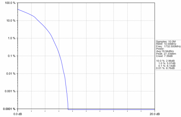
Band4_10MHz_16QAM_MCH_1732.5MHz_RB_27_0_NTNV
