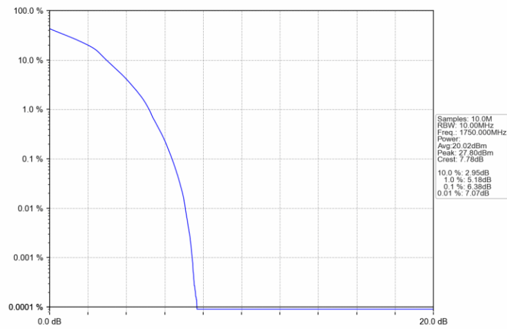
Band4_10MHz_16QAM_HCH_1750MHz_RB_27_23_NTNV
