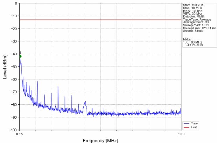
Band4_1.4MHz_QPSK_LCH_1710.7MHz_RB_1_0_NTNV
