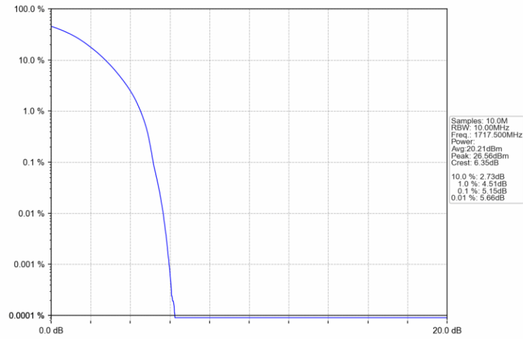
Band4_15MHz_QPSK_LCH_1717.5MHz_RB_75_0_NTNV
