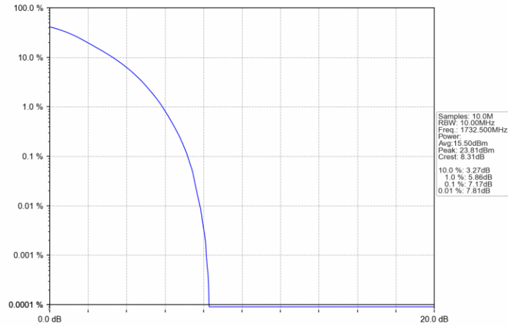
Band4_20MHz_16QAM_MCH_1732.5MHz_RB_27_0_NTNV
