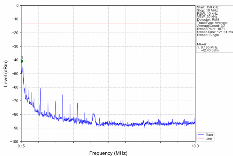
Band4_5MHz_16QAM_LCH_1712.5MHz_RB_1_0_NTNV
