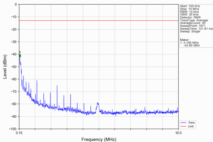
Band4_15MHz_16QAM_LCH_1717.5MHz_RB_1_0_NTNV
