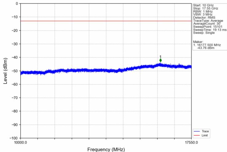
Band4_20MHz_16QAM_MCH_1732.5MHz_RB_1_0_NTNV
