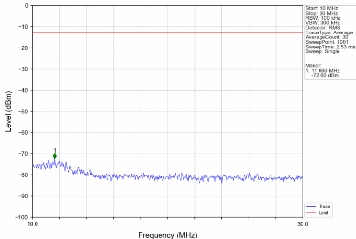
Band4_15MHz_16QAM_LCH_1717.5MHz_RB_1_0_NTNV
