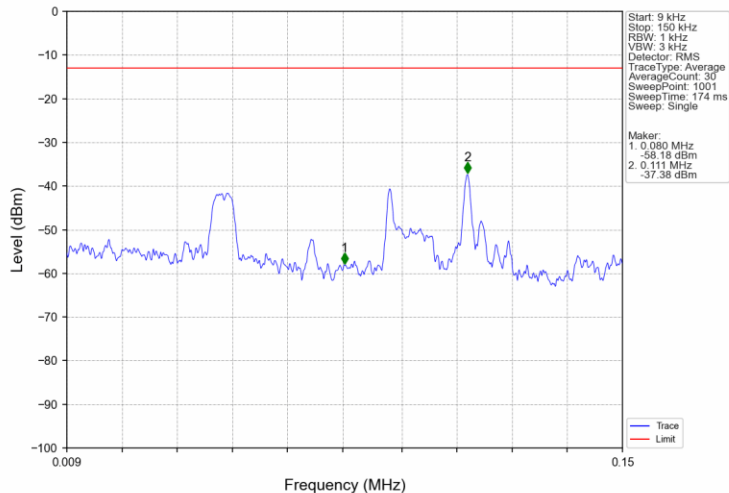
Band4_15MHz_16QAM_LCH_1717.5MHz_RB_1_0_NTNV
