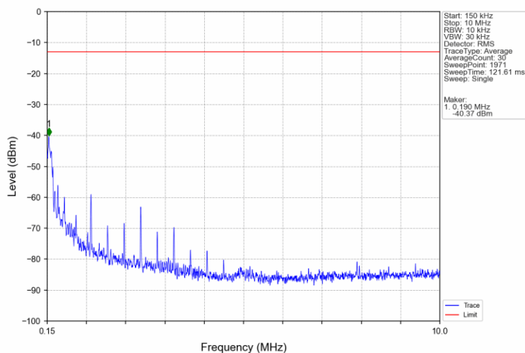
Band66_3MHz_16QAM_MCH_1745MHz_RB_1_0_NTNV
