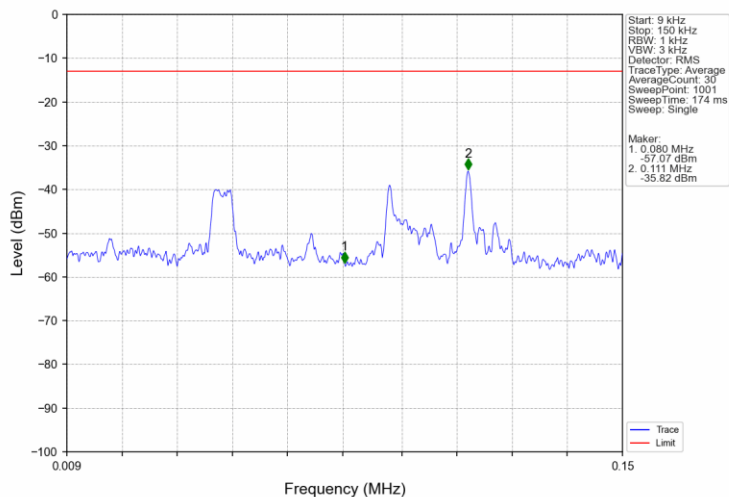
Band66_3MHz_16QAM_MCH_1745MHz_RB_1_0_NTNV
