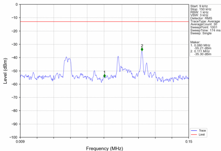
Band66_15MHz_16QAM_LCH_1717.5MHz_RB_1_0_NTNV
