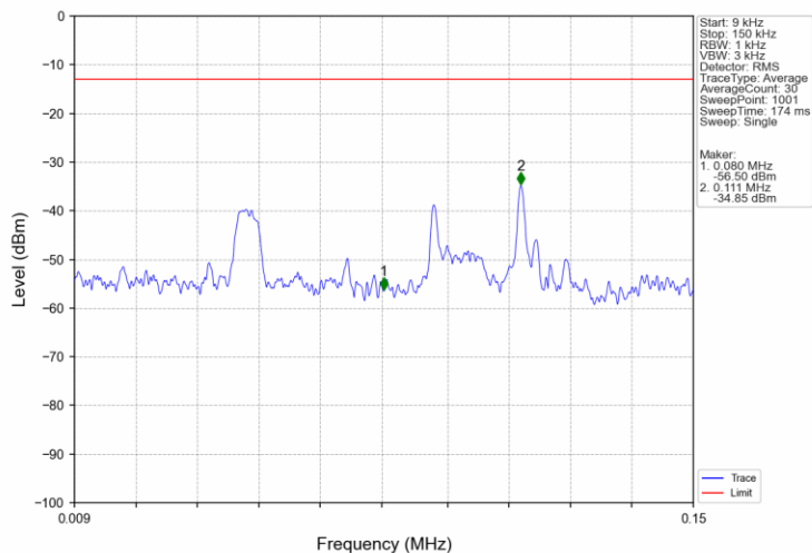
Band66_20MHz_16QAM_HCH_1770MHz_RB_1_0_NTNV
