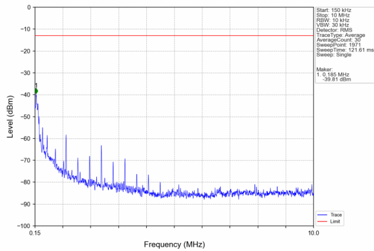
Band66_15MHz_16QAM_HCH_1772.5MHz_RB_1_0_NTNV
