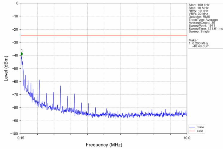
Band7 5MHz 16QAM LCH 2502.5MHz RB 1 0 NTV
