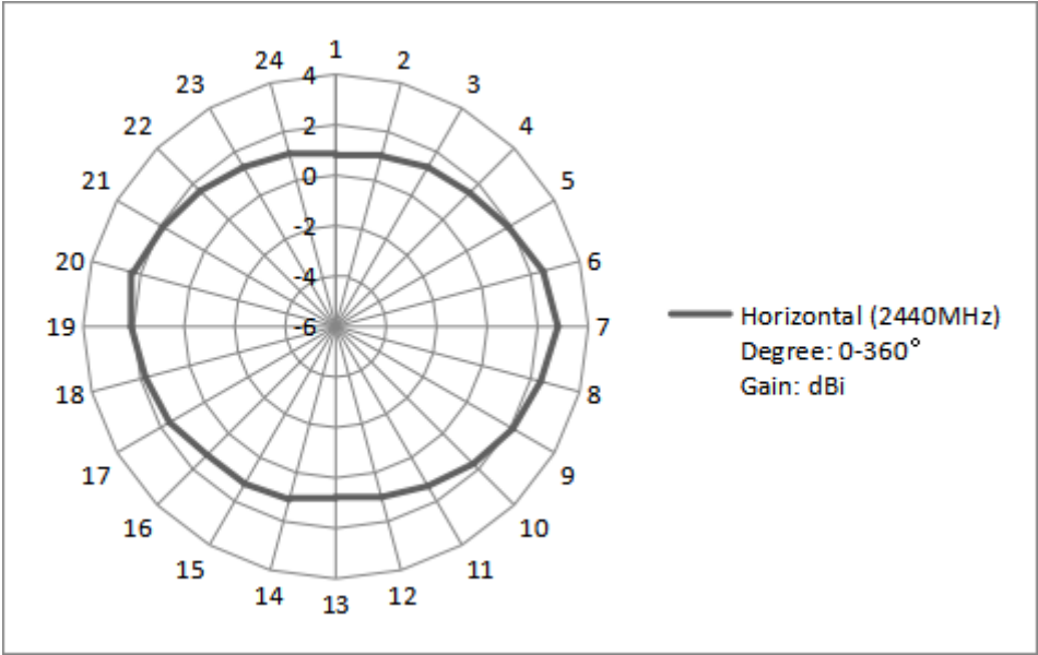
Horizontal (2440MHz) Degree: 0-360° Gain: dBi
