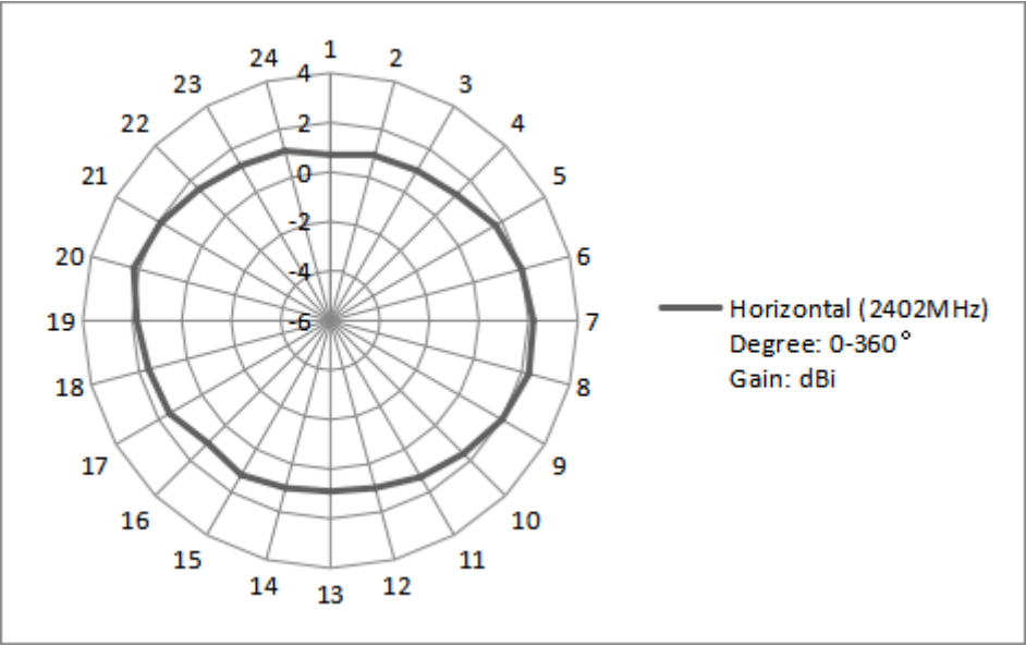
Horizontal (2402MHz) Degree: 0-360° Gain: dBi
