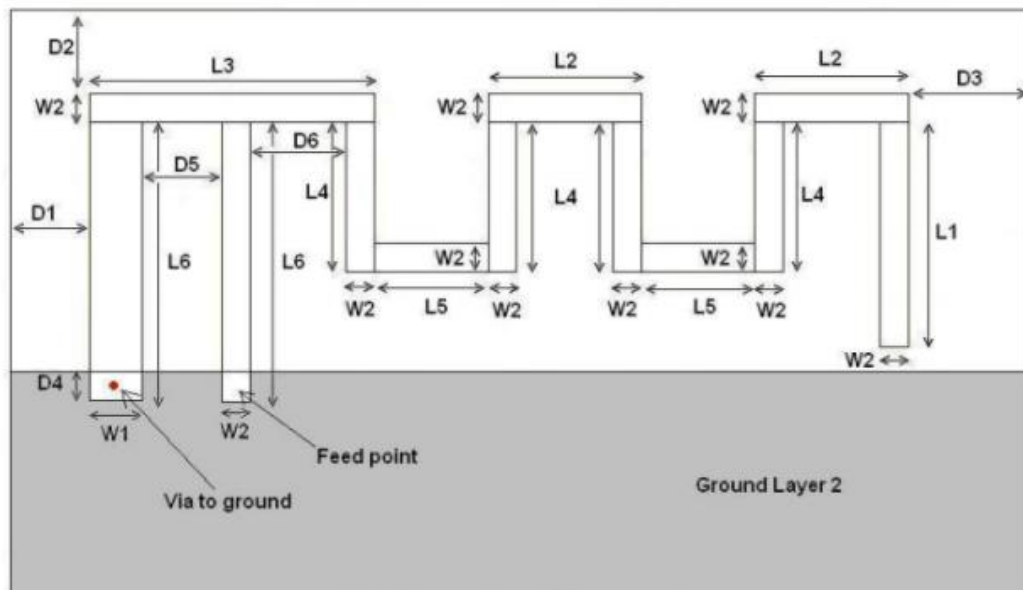
Figure 3: Antenna Dimensions
