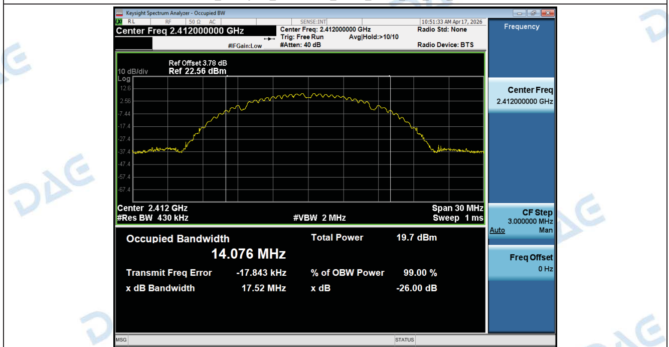
99%_Occupied_Bandwidth_NVNT_ANT1_802_11b_2412
