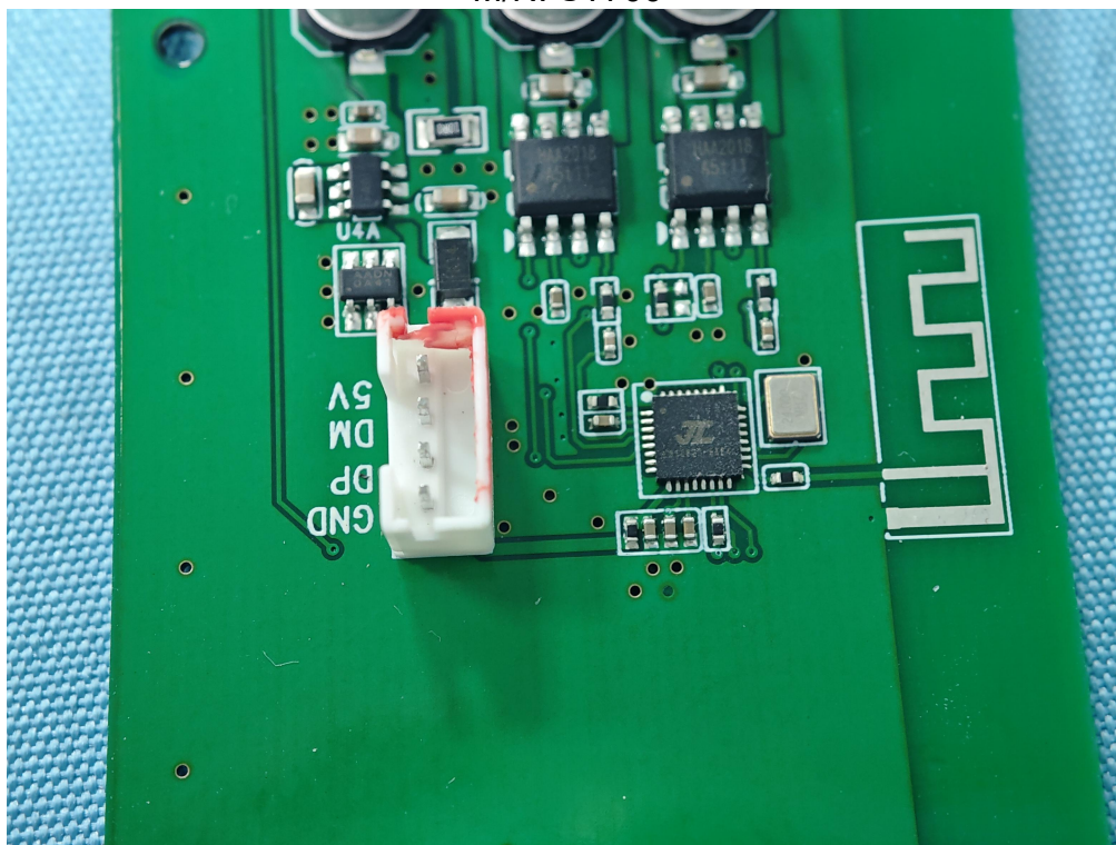
Photo 4 Internal photos of EUT M/N: ST700
