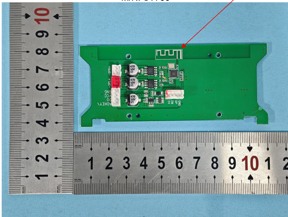
Photo 2 Internal photos of EUT M/N: ST700
