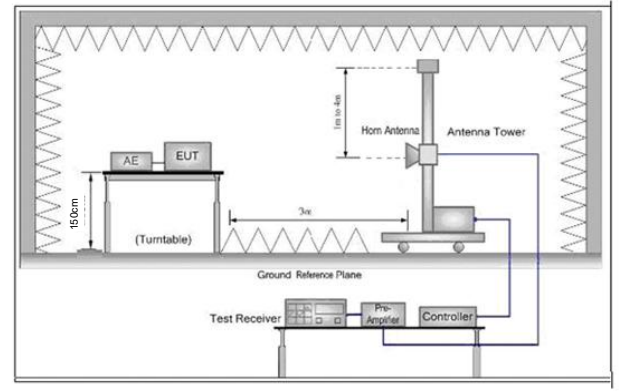
Figure 3. Above 1 GHz
