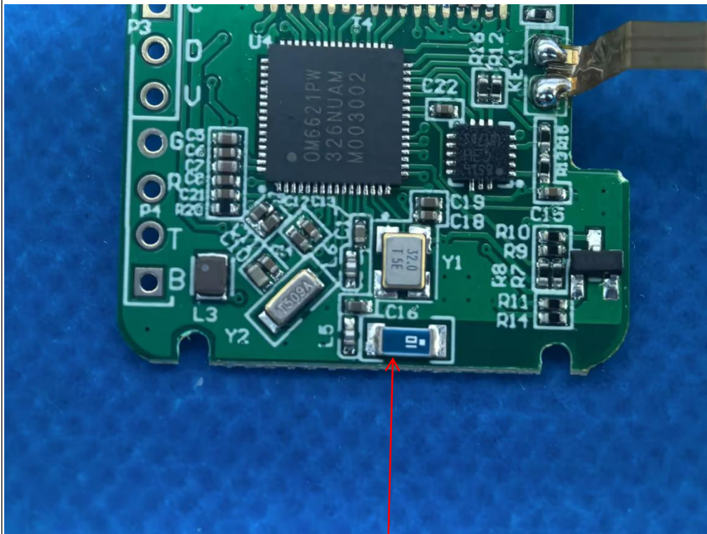
Ceramic Antenna
