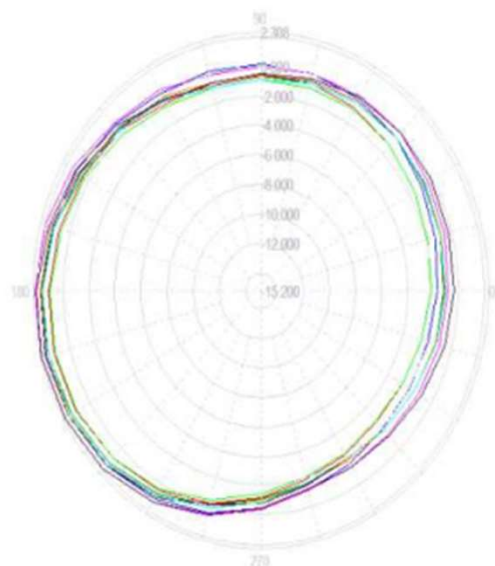
H Plane PolarLine Chart
