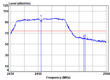
11n_HT(40M)_TX_CH_09_Vertical-Peak
