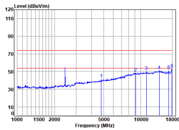
BLE_1M_TX_CH_19_Horizontal
