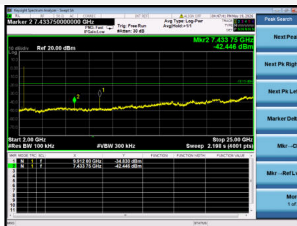
GFSK (BLE 2Mbps) HIGH CHANNEL, SPURIOUS 2 GHz ~ 25 GHz
