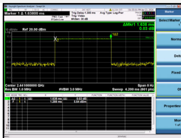
8-DPSK 3DH3
