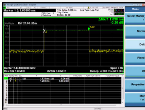
GFSK DH3
