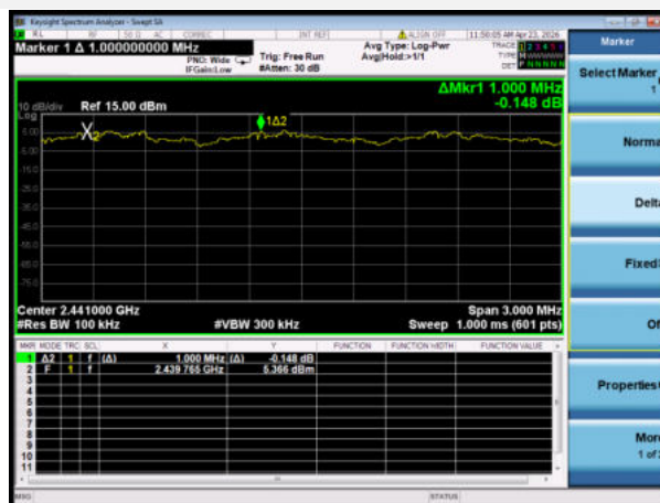
8-DPSK
