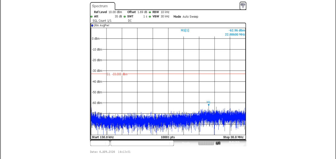
Band4-1513-3-0.15~30MHz-PASS
