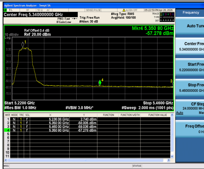
11AX20SISO_Ant2_High_5240_Peak
