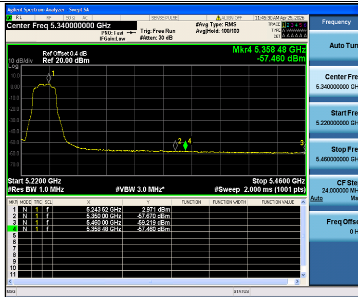
11AX20SISO_Ant2_High_5240_Peak
