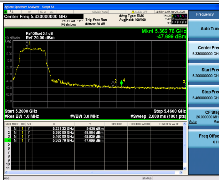
11AX40SISO_Ant2_High_5230_Peak
