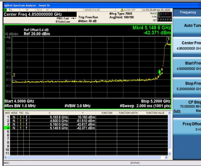
11AX40SISO_Ant2_High_5230_AV
