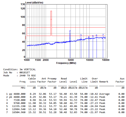
2.4G_SRD_MID_TX_Vertical
