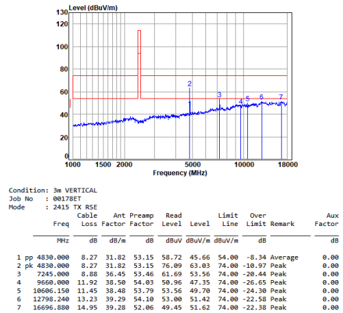
2.4G_SRD_LOW_TX_Vertical
