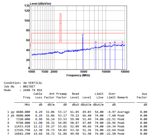
2.4G_SRD_MID_TX_Vertical
