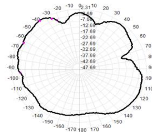
5790.0MHz Total(E1), Max= 0.62dBi
