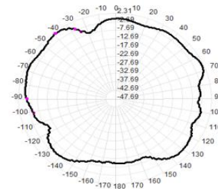
5790.0MHz Total(E2), Max= 2.63dBi
