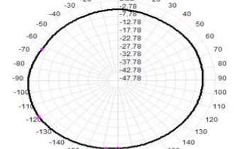
2400.0MHz Total(H), Max= -1.62dBi
