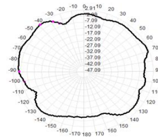
2470.0MHz Total(E2), Max= 2.29dBi
