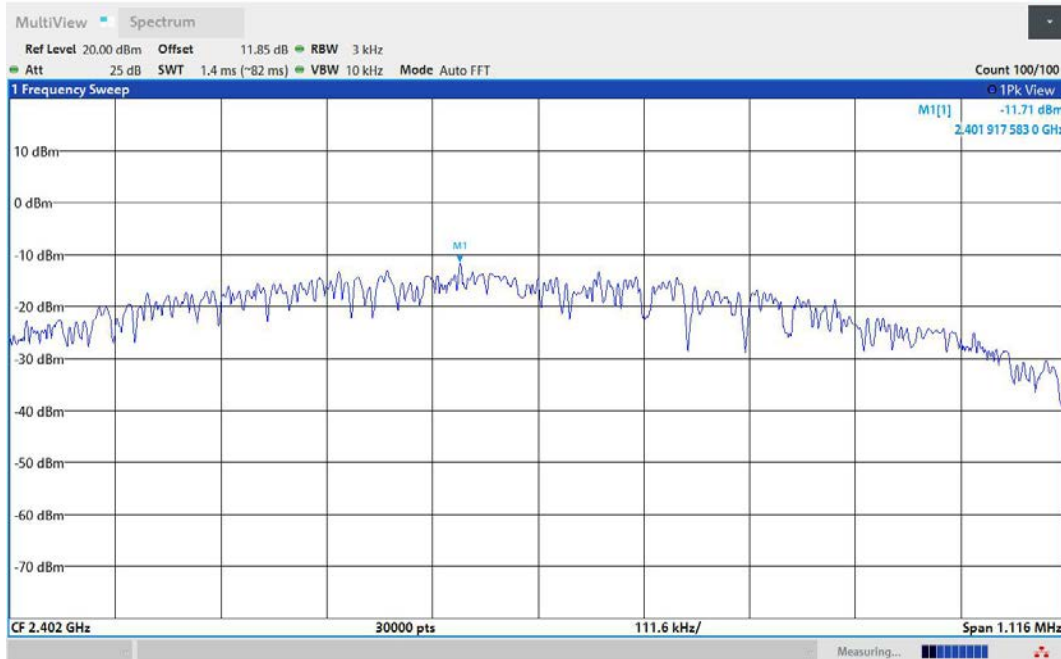
BLE_1M-Ant1-2402-PASS
