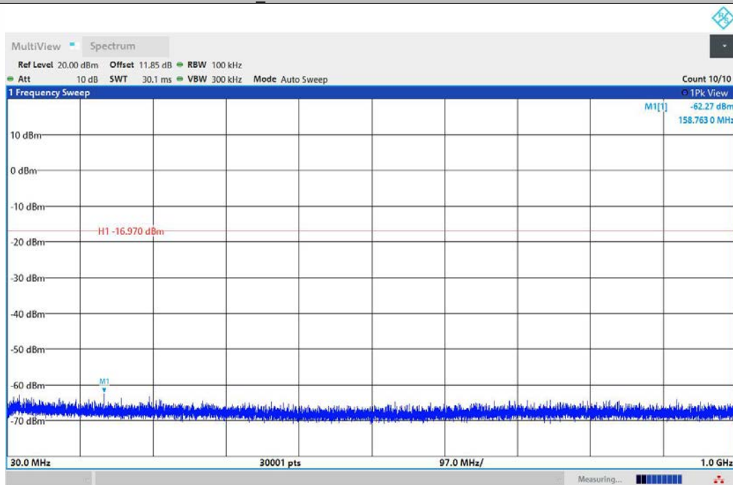
BLE_1M-Ant1-2402-30~1000-PASS
