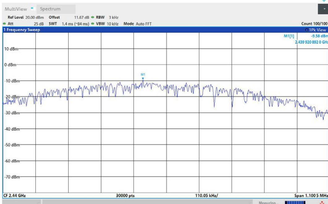
BLE_1M-Ant1-2440-PASS
