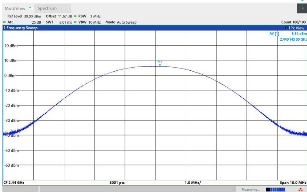
BLE_1M-Ant1-2440-PASS
