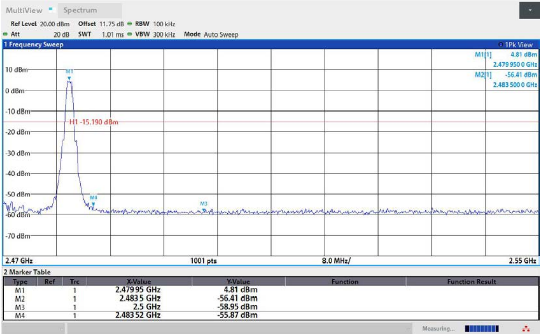
BLE_1M-Ant1-2480-PASS
