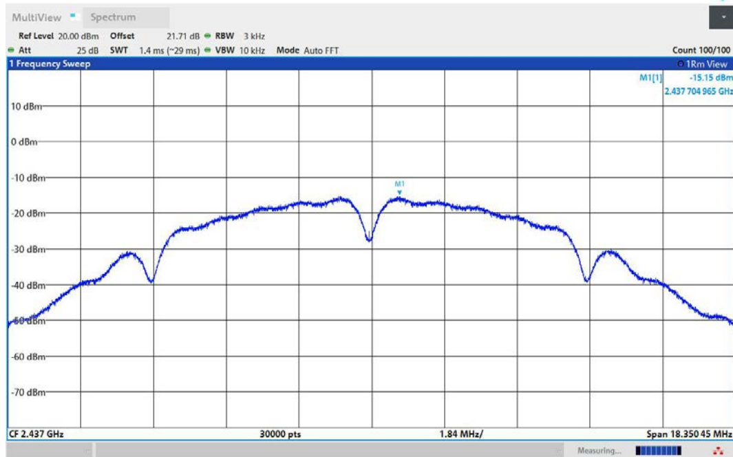
11B-Ant1-2437-PASS
