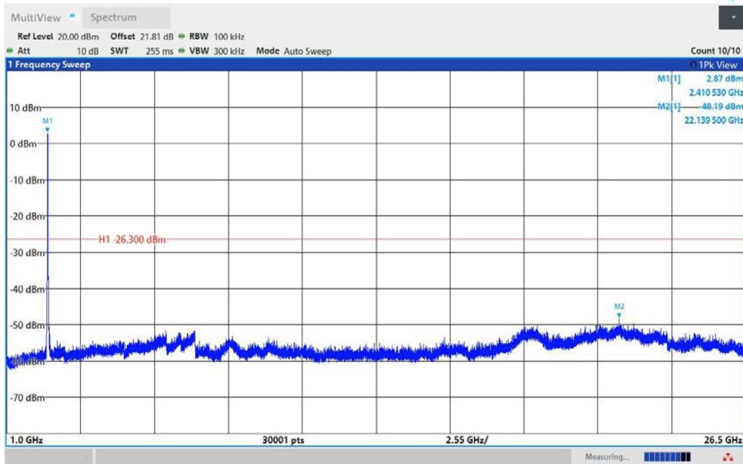
11N20SISO-Ant1-2412-1000~26500-PASS
