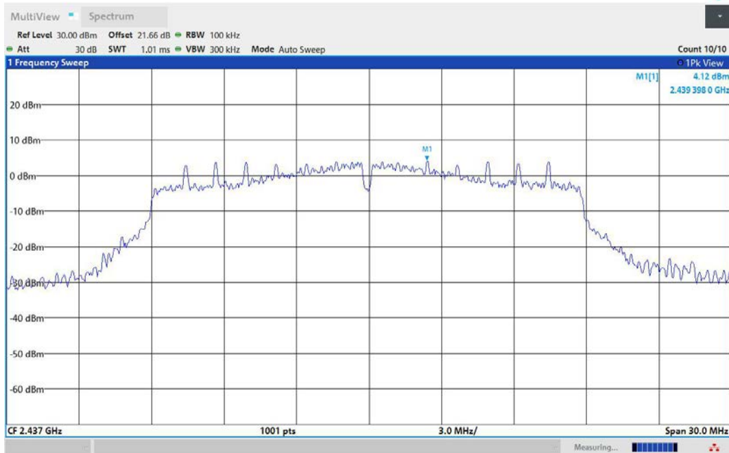
11N20SISO-Ant1-2437-0~Reference-PASS
