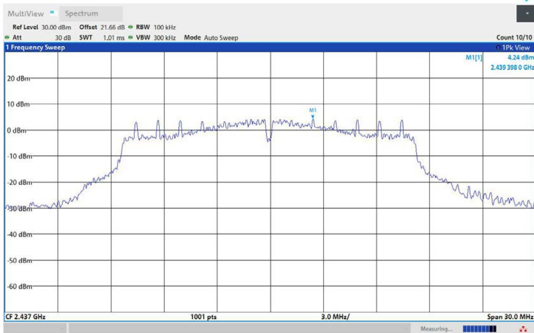
11G-Ant1-2437-0~Reference-PASS
