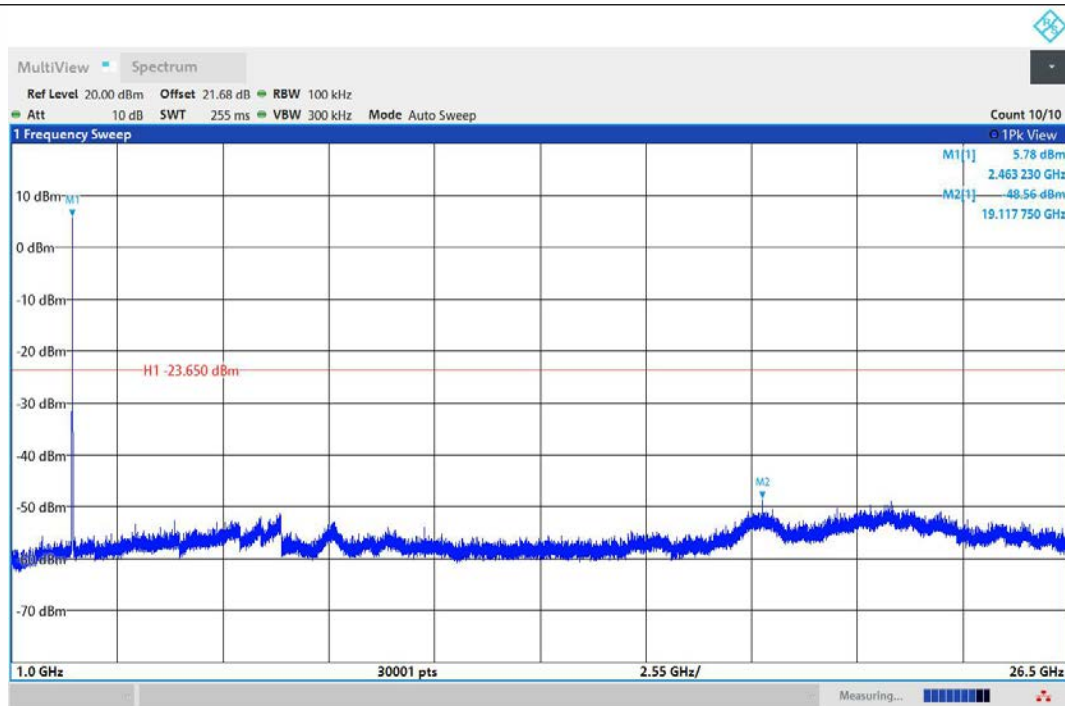
11B-Ant1-2462-1000~26500-PASS
