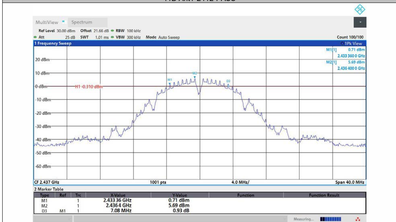
11B-Ant1-2437-PASS
