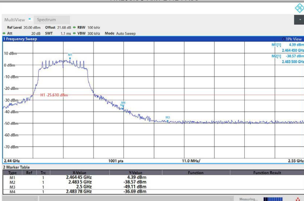
11N20SISO-Ant1-2462-PASS
