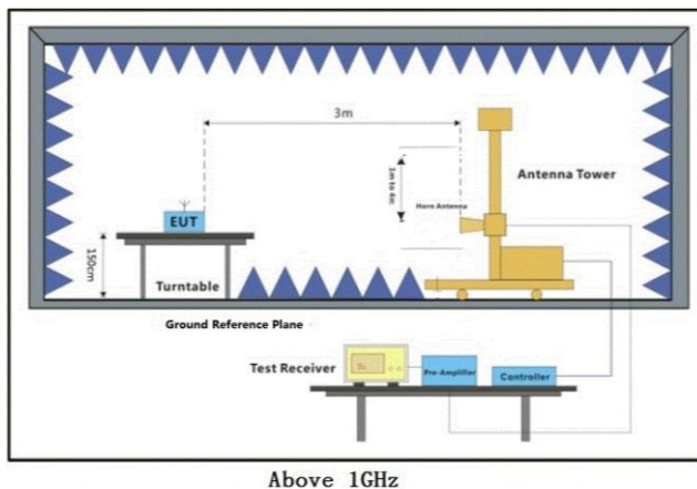
Above 1GHz
