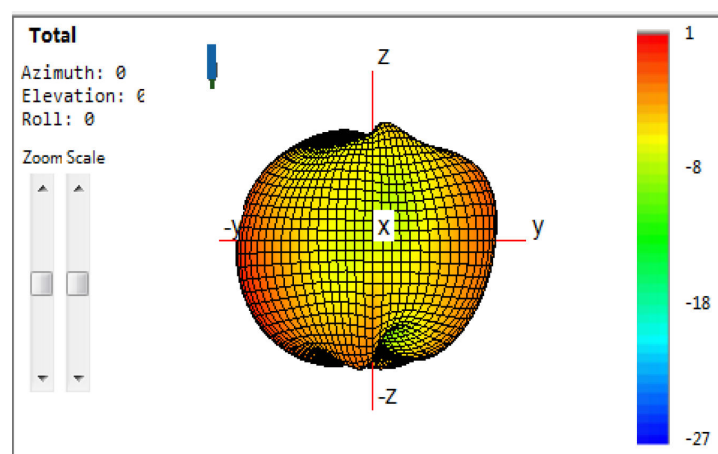
Antenna Radiation Pattern-3D
