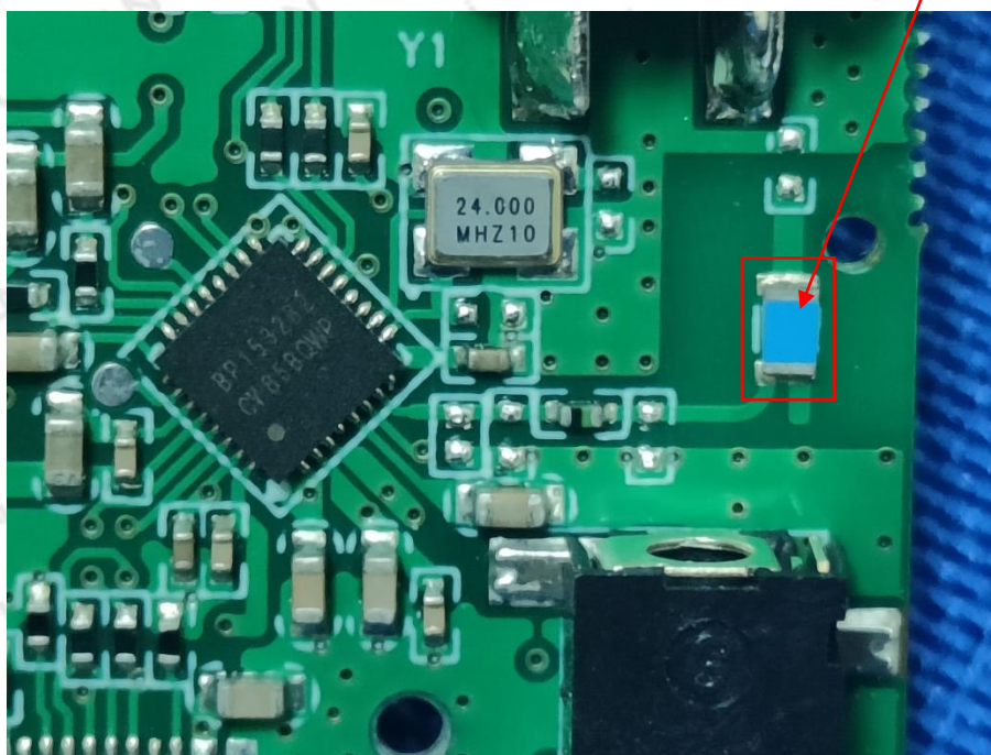
Chip Antenna
